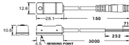
UL-21N(P)-03 UL-21N(P)-QC8
